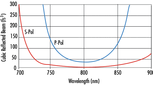
Ultrafast Ti:Sapphire Laser Mirror Cubic Term
