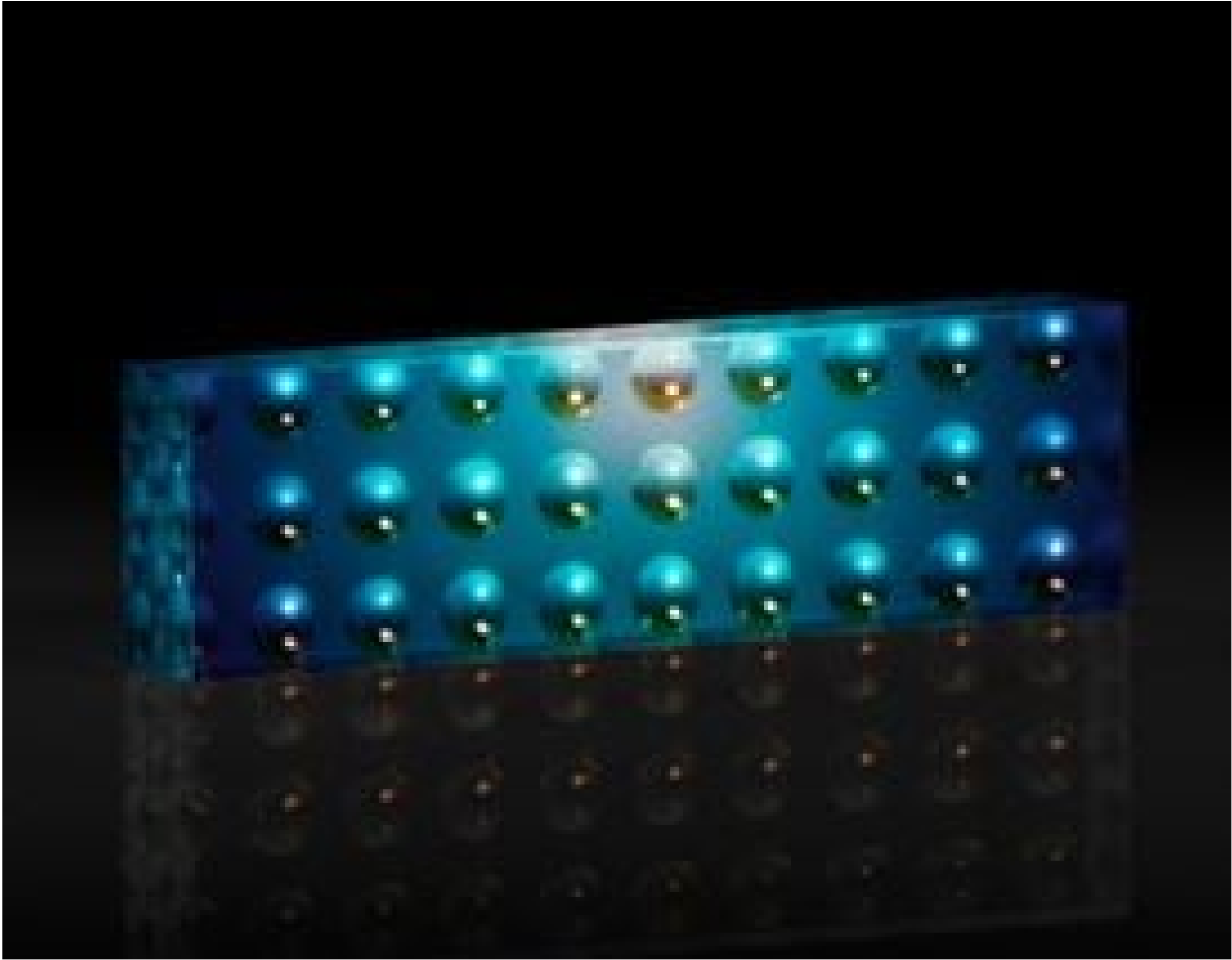
#21-175, 7.30 x2.05mm, 0.575 ROC, 750µm Pitch, 1 x8 Linear Micolens Array
