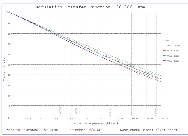
#36-366, 8.0mm FL f/5.6 Rugged Blue Series M12 Lens, Modulated Transfer Function (MTF) Plot, 150mm Working Distance, f5.6
