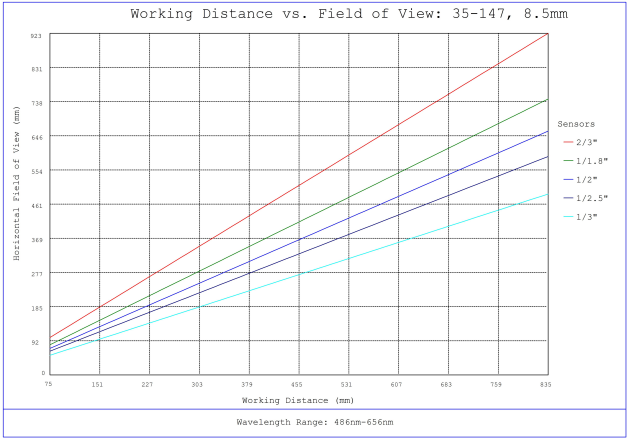
#35-147, 8.5mm, f/1.8, 75mm-∞ Primary WD, HRr Series Fixed Focal Length Lens, Working Distance versus Field of View Plot
