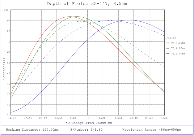
#35-147, 8.5mm, f/1.8, 75mm-∞ Primary WD, HRr Series Fixed Focal Length Lens, Depth of Field Plot, 150mm Working Distance, f1.8
