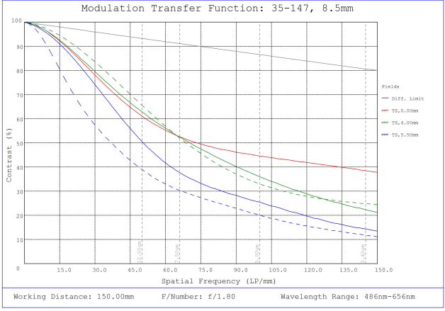
#35-147, 8.5mm, f/1.8, 75mm-∞ Primary WD, HRr Series Fixed Focal Length Lens, Modulated Transfer Function (MTF) Plot, 150mm Working Distance, f1.8
