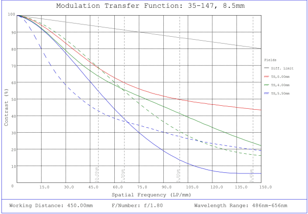
#35-147, 8.5mm, f/1.8, 75mm-∞ Primary WD, HRr Series Fixed Focal Length Lens, Modulated Transfer Function (MTF) Plot, 450mm Working Distance, f1.8
