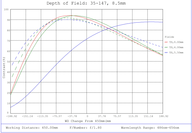
#35-147, 8.5mm, f/1.8, 75mm-∞ Primary WD, HRr Series Fixed Focal Length Lens, Depth of Field Plot, 450mm Working Distance, f1.8
