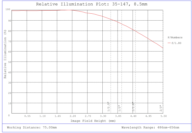
#35-147, 8.5mm, f/1.8, 75mm-∞ Primary WD, HRr Series Fixed Focal Length Lens, Relative Illumination Plot
