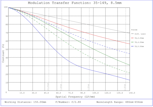
#35-149, 8.5mm, f/2.8, 75mm-∞ Primary WD, HRr Series Fixed Focal Length Lens, Modulated Transfer Function (MTF) Plot, 150mm Working Distance, f2.8
