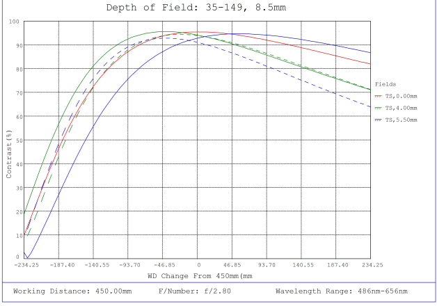
#35-149, 8.5mm, f/2.8, 75mm-∞ Primary WD, HRr Series Fixed Focal Length Lens, Depth of Field Plot, 450mm Working Distance, f2.8
