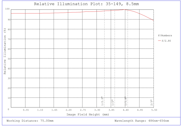
#35-149, 8.5mm, f/2.8, 75mm-∞ Primary WD, HRr Series Fixed Focal Length Lens, Relative Illumination Plot
