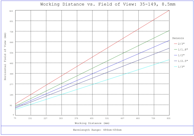
#35-149, 8.5mm, f/2.8, 75mm-∞ Primary WD, HRr Series Fixed Focal Length Lens, Working Distance versus Field of View Plot
