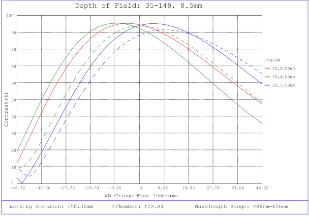
#35-149, 8.5mm, f/2.8, 75mm-∞ Primary WD, HRr Series Fixed Focal Length Lens, Depth of Field Plot, 150mm Working Distance, f2.8
