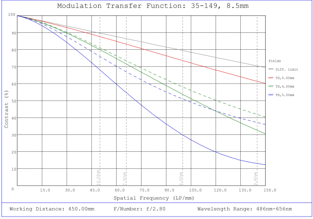
#35-149, 8.5mm, f/2.8, 75mm-∞ Primary WD, HRr Series Fixed Focal Length Lens, Modulated Transfer Function (MTF) Plot, 450mm Working Distance, f2.8
