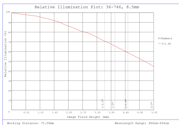
#36-746, 8.5mm f/1.4, 75mm- \infty Primary WD, HRi Series Fixed Focal Length Lens, Relative Illumination Plot
