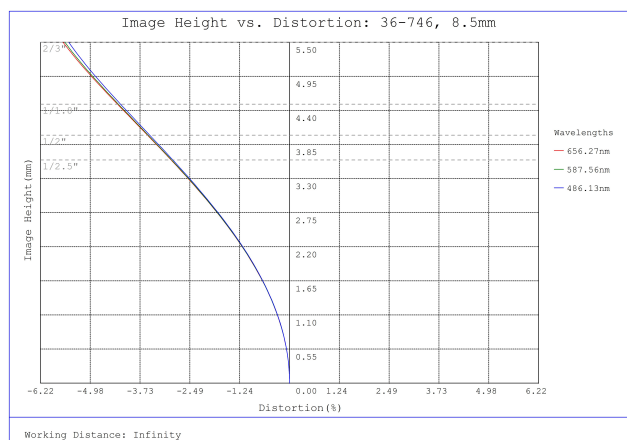
#36-746, 8.5mm f/1.4, 75mm- \infty Primary WD, HRi Series Fixed Focal Length Lens, Distortion Plot
