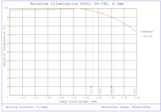
#36-748, 8.5mm f/2, 75mm-∞ Primary WD, HRI Series Fixed Focal Length Lens, Relative Illumination Plot
