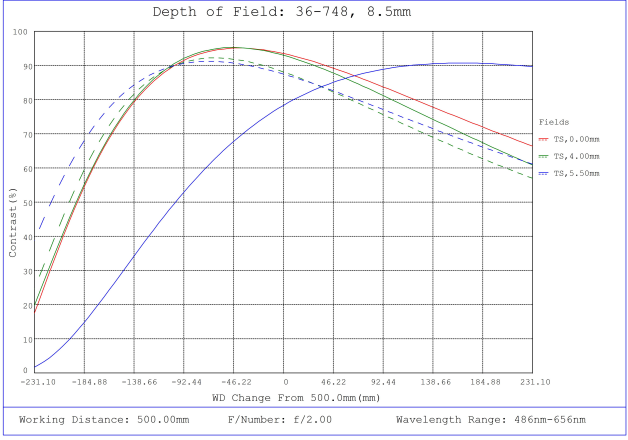
#36-748, 8.5mm f/2, 75mm-∞ Primary WD, HRi Series Fixed Focal Length Lens, Depth of Field Plot, 500mm Working Distance, f2
