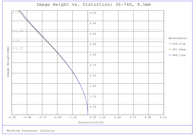
#36-748, 8.5mm f/2, 75mm-∞ Primary WD, HRI Series Fixed Focal Length Lens, Distortion Plot
