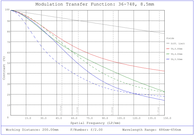
#36-748, 8.5mm f/2, 75mm-∞ Primary WD, HRi Series Fixed Focal Length Lens, Modulated Transfer Function (MTF) Plot, 200mm Working Distance, f2
