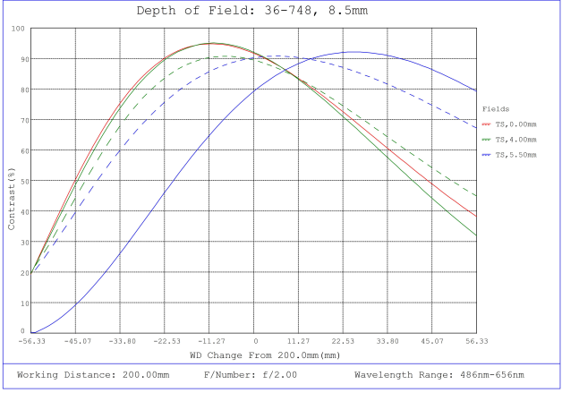
#36-748, 8.5mm f/2, 75mm-∞ Primary WD, HRi Series Fixed Focal Length Lens, Depth of Field Plot, 200mm Working Distance, f2
