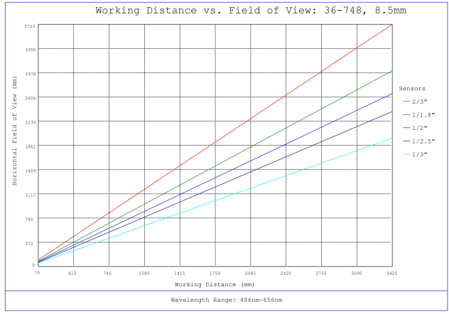
#36-748, 8.5mm f/2, 75mm-∞ Primary WD, HRI Series Fixed Focal Length Lens, Working Distance versus Field of View Plot
