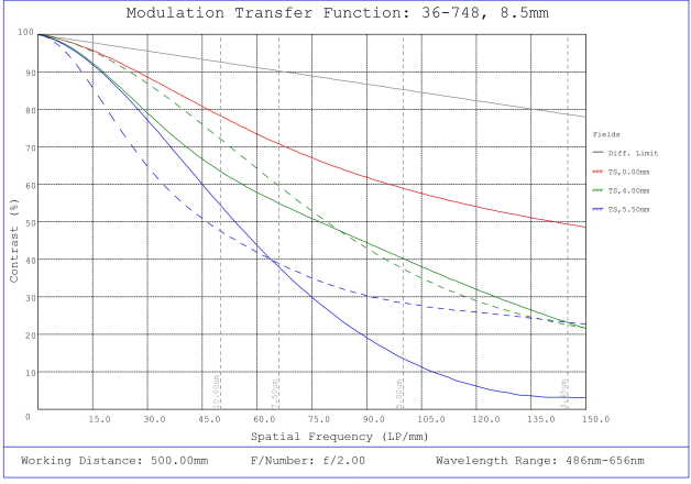
#36-748, 8.5mm f/2, 75mm-∞ Primary WD, HRi Series Fixed Focal Length Lens, Modulated Transfer Function (MTF) Plot, 500mm Working Distance, f2
