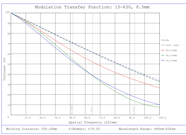
#15-630, 8.5mm, f/8 Cw Series Fixed Focal Length Lens, Modulated Transfer Function (MTF) Plot, 500mm Working Distance, f8
