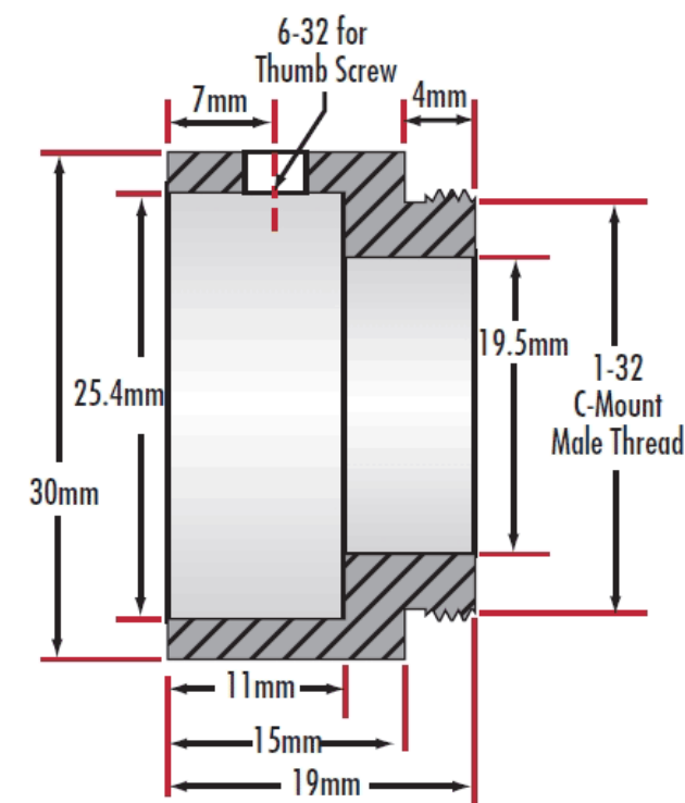
C-Mount Dimensions
