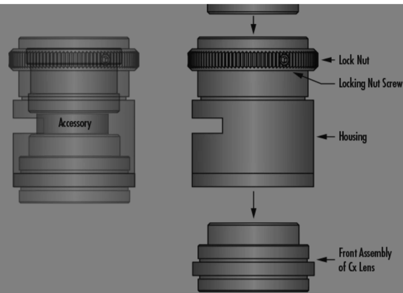
Cx Lens Assembly Diagram
