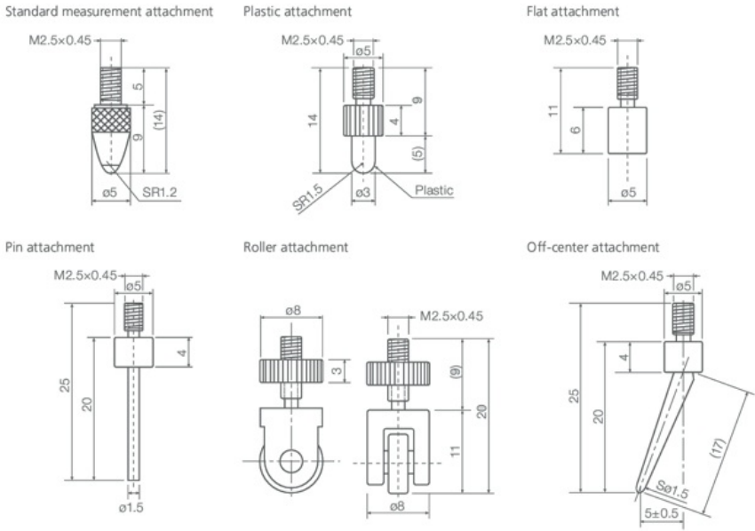
PID4485_Measurement_Probes
