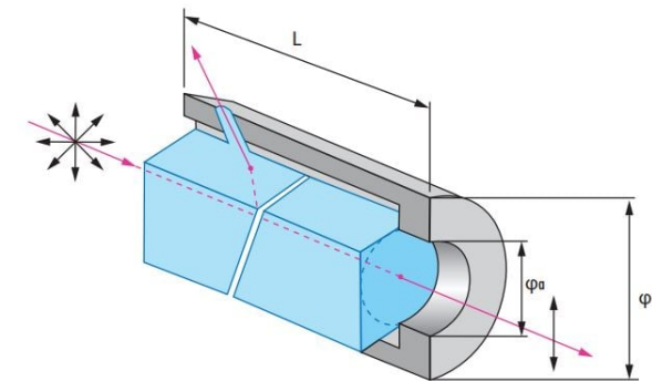
Glan-Laser Polarizers
