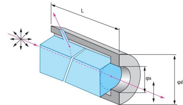
Glan-Laser Polarizers
