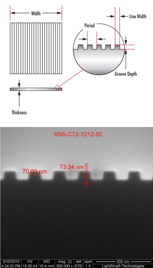
SEM Image of 139nm, 50nm Groove Depth Linear Silicon Nanostamps (Cross Section)
