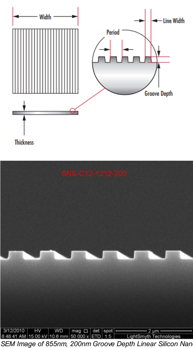
SEM Image of 855nm, 200nm Groove Depth Linear Silicon Nanostamps (Cross Section)
