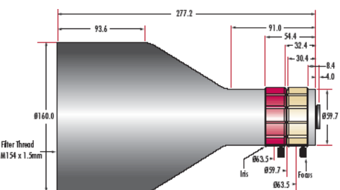
0.08X & 0.06X Telecentric Lens Units: mm
