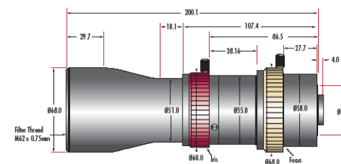
1X & 0.73X Telecentric Lenses Units: mm
