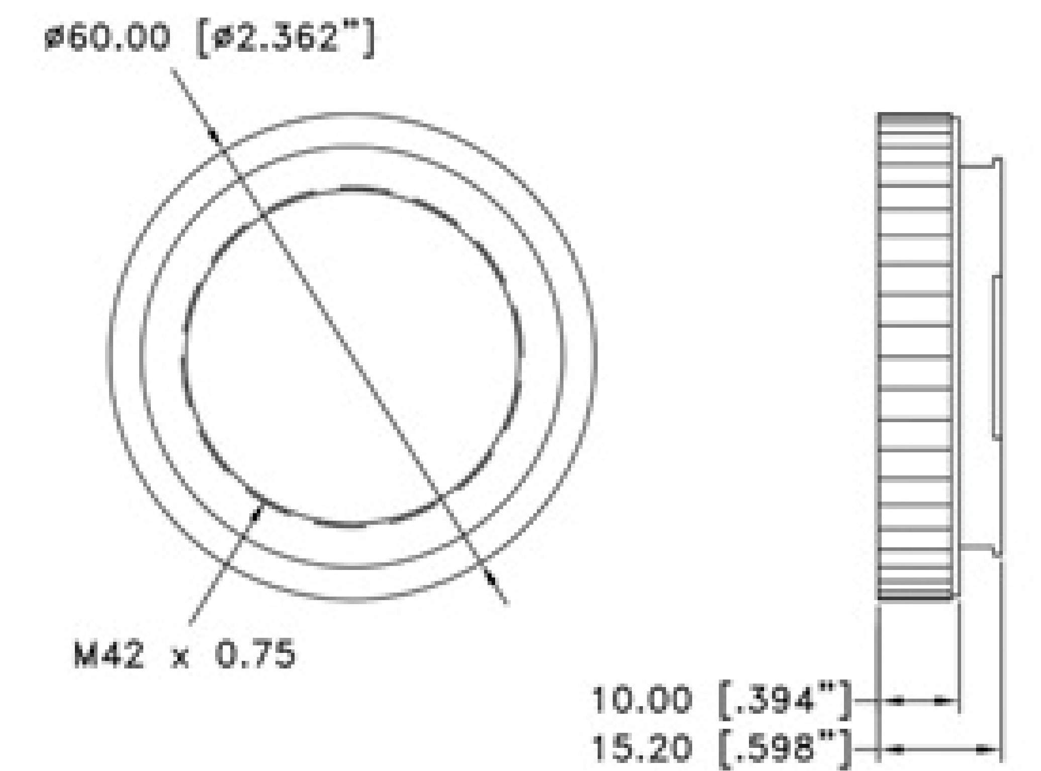
#16-139: T-Mount (M42) to Sony A Mount
