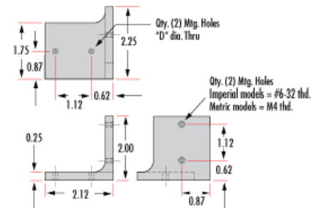
1.75" Z-Axis Adapter Plate (#54-374)
